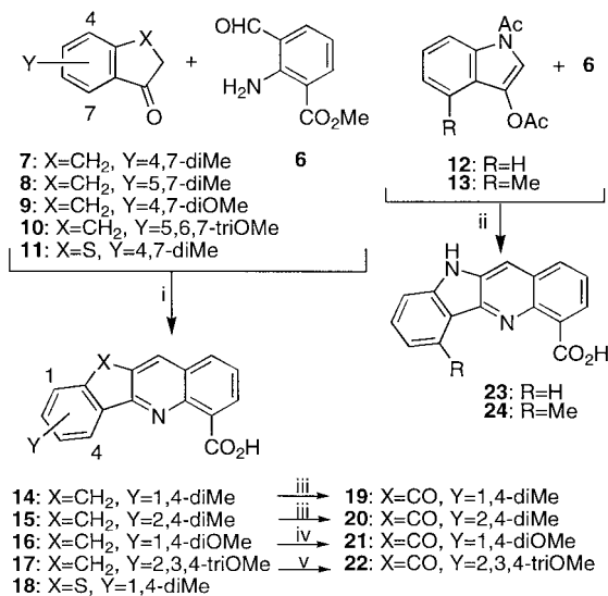
Scheme 1. (i) t -BuOK/ t -BuOH ( 14–16 ), piperidine/EtOH ( 18 ); (ii) NaOH/aq. EtOH; (iii) Na 2 Cr 2 O 7 /3 M H 2 SO 4 ; (iv) SeO 2 /dioxan; (v) KMnO 4 /aq. Na 2 CO 3 .
